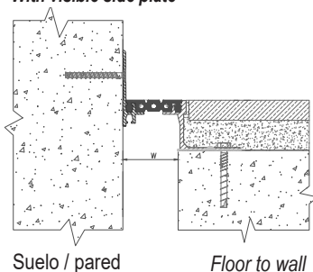
JDH 5.02-060 A con cantonera visible With visible side plate
