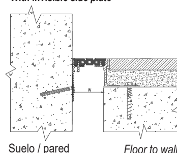
JDH 5.02-060 A con cantonera invisible With invisible side plate
