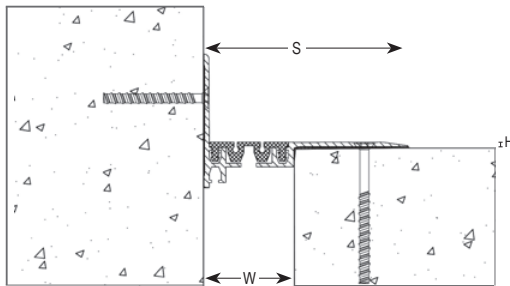
JDH 5.26-050 A (Angle) visible side part
