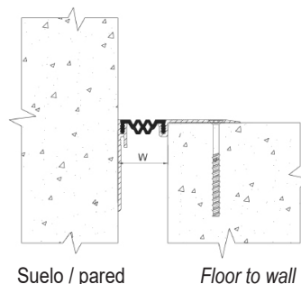
JDH 5.26-040 A con laterale invisible / With invisible side plate
