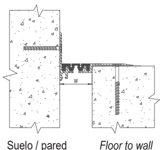
JDH 5.26-050 A con laterale visible / With visible side plate
