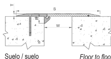
JDH 6.35-075 a / to 100
