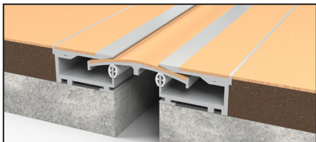
JDH 6.26-050 A con cantonera visible With invisible side plate
