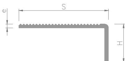
NDM VDi strié / striped NDM VDi
