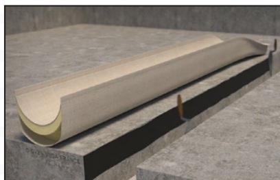
Apply the VEDACOLLE ® adhesive to the inside edges of the joint on a depth of 90mm.
